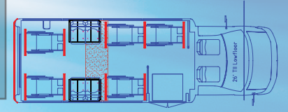
26', 5 Wheelchair Positions, 17 Passengers
