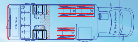
28', 3 Wheelchair Positions, 9 Passengers
