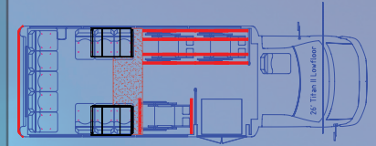
26', 3 Wheelchair Positions, 11 Passengers
